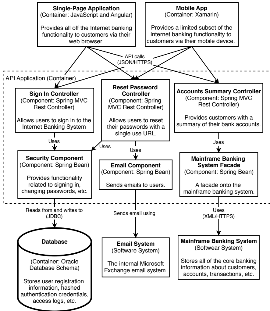
Figure C.3 A component diagram. Image adapted from https://c4model.com/ , licensed under https://creativecommons.org/licenses/by/4.0/ .
