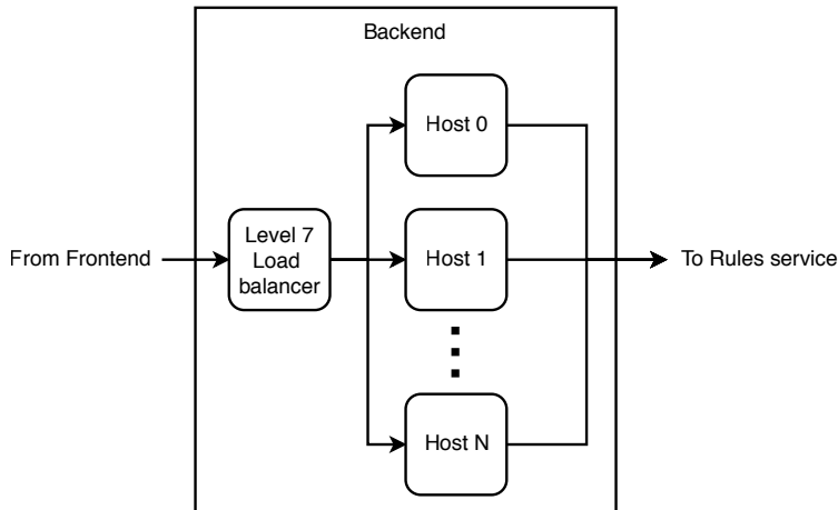
Figure 8.5 Backend architecture of rate limiter that employs a stateful sharded approach. The counts are stored in the hosts' memory, rather than in a distributed cache like Redis.
