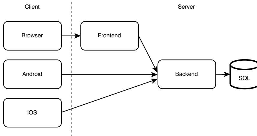
Figure 1.1 Initial system design of our app. For a more thorough discussion on the rationale for having three client applications and two server applications (excluding the SQL application/database), refer to chapter 6.
