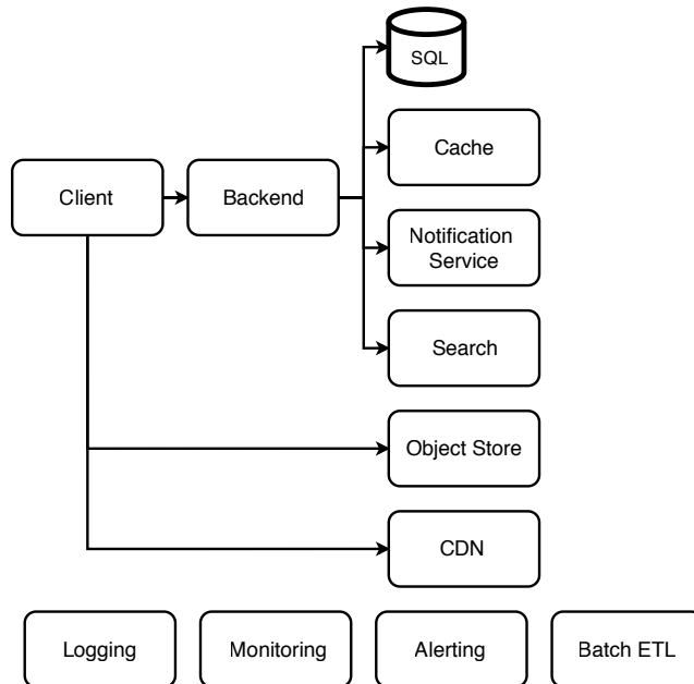
Figure 7.9 Our Craigslist architecture with notification service, search, logging, monitoring, and alerting. Logging, monitoring, and alerting can serve many other components, so on our diagram, they are shown as loose components. We can define jobs on the batch ETL service for purposes such as to periodically remove old posts.
