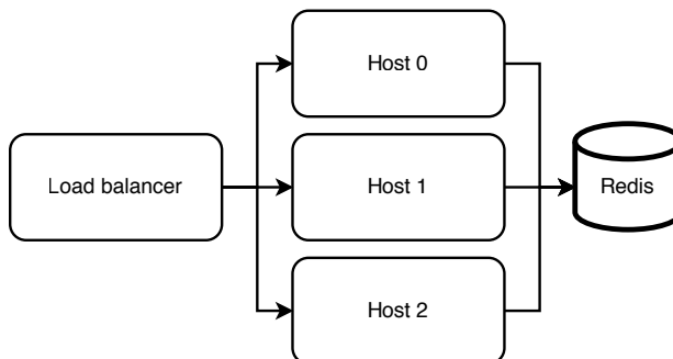
Figure 4.8 We can replace a node with a service, which we refer to as an aggregation unit. This unit has three stateless hosts for fault-tolerance, but we can use more hosts if desired.
