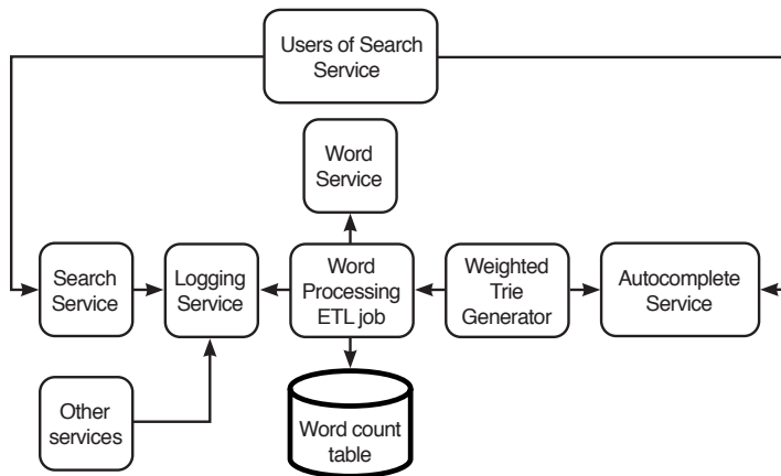
Figure 11.2 Initial high-level architecture of our Autocomplete System. Users of our search service submit their search strings to the search service, and these strings are logged to a shared logging service. The Word Processing ETL job may be a batch or streaming job that reads and processes the logged search strings. The weighted trie generator reads the word counts and generates the weighted trie and then sends it to the autocomplete service, from which users obtain autocomplete suggestions.
