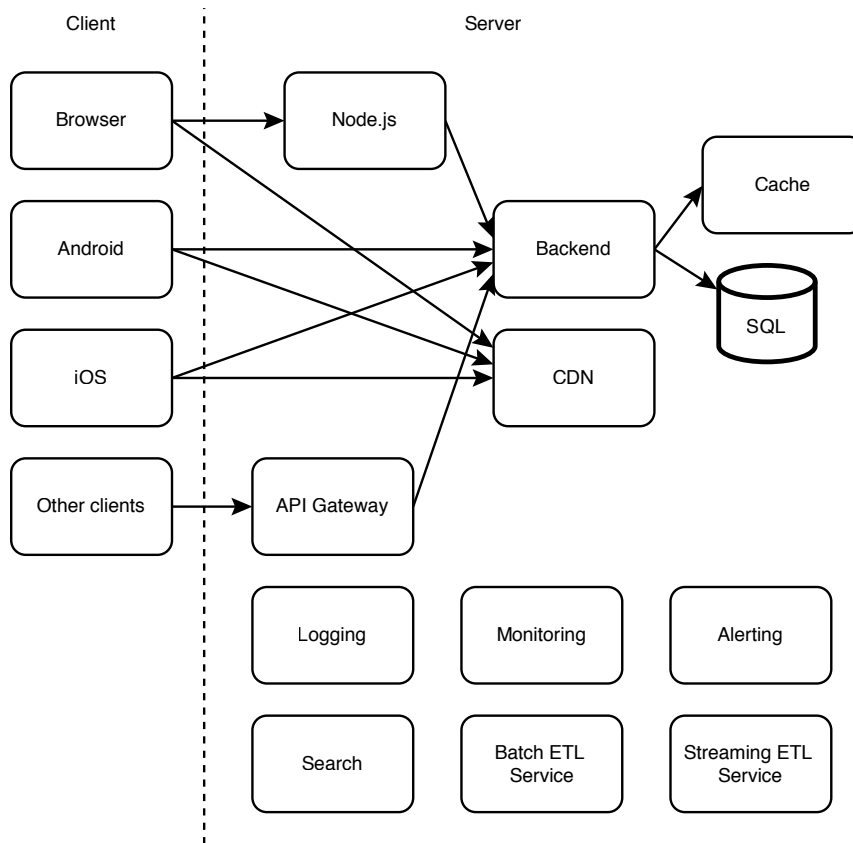
Figure 1.7 Initial architecture with our API gateway and services. Requests to services go through the API gateway
