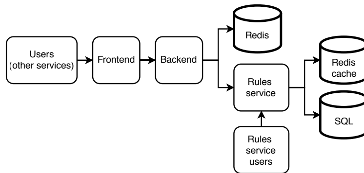
Figure 8.4 Rate limiter with Redis cache on the Rules service. Frequent requests from the backend can be served from this cache instead of the SQL database.
