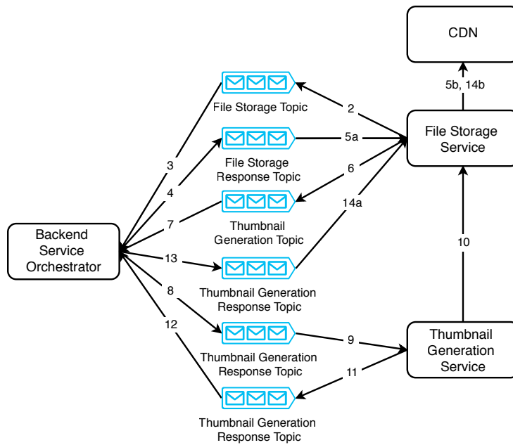
Figure 12.6 Orchestration of thumbnail generation, starting from step 2. Figure 12.5 illustrated the object storage service, which we omit on this diagram for brevity. For clarity, we also don't illustrate the user.
