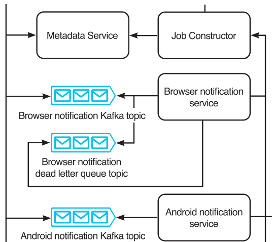
Figure 9.12 Zoom-in of figure 9.6, with the addition of a browser notification dead letter queue. The dead letter queues for the other channel services will be similar. If the browser notification service encounters a 503 Service Unavailable error when delivering a notification, it produces/enqueues this notification event to its dead letter queue. It will retry the delivery later. If delivery fails after three attempts, the browser notification service will log the event (to our shared logging service). We may also choose to also configure a low-urgency alert for such failed deliveries.
