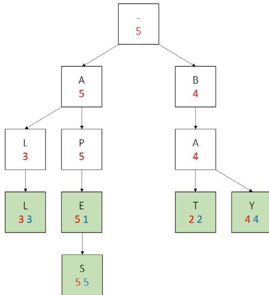
Figure 11.3 A weighted trie of the words “all”, “apes,” “bat,” and “bay.” (Source: https://courses.cs.duke.edu/cps100/spring16/autocomplete/trie.html .)
