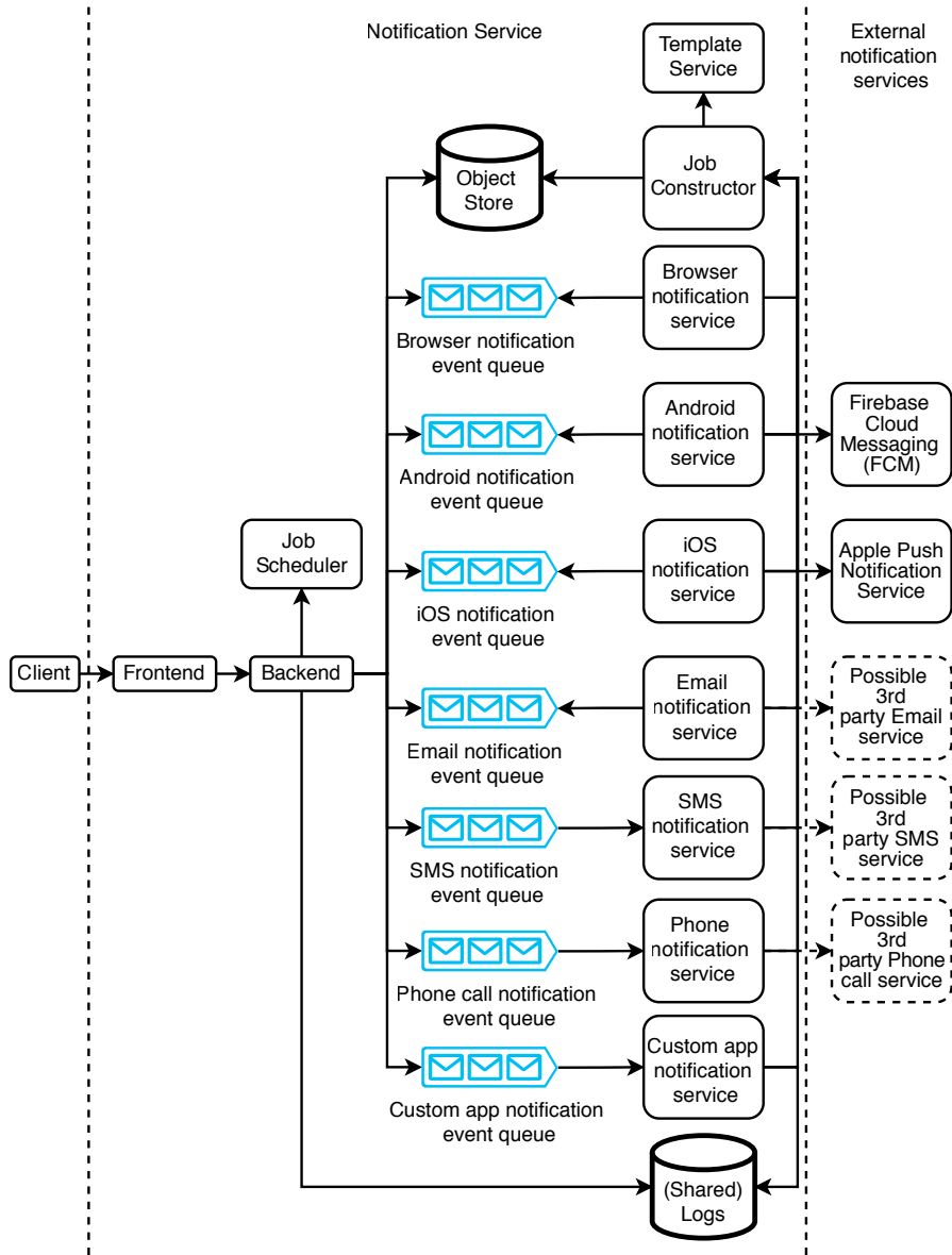
Figure 9.7 High-level architecture with an Airflow/job scheduler service. The job scheduler service is for users to configure periodic notifications. At the scheduled times, the job scheduler service will produce notification events to the backend.
