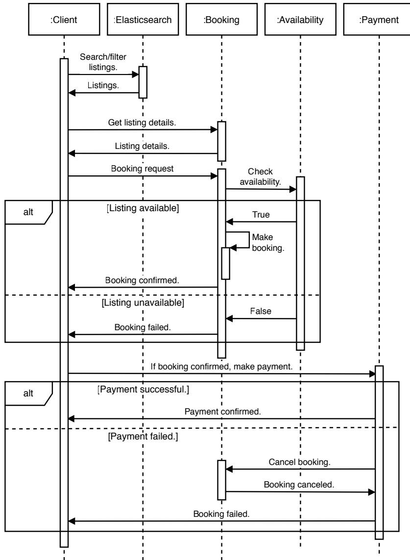
Figure 15.9 Sequence diagram of our simplified booking process. Many details are glossed over. Examples: Getting the listing details may involve a CDN. We don't give hosts the option to manually accept or reject booking requests. Making payment will involve a large number of requests to multiple services. We did not illustrate requests to our notification service.
