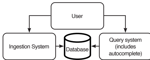
Figure 11.1 A very high-level initial architecture of our autocomplete service. Users submit their strings to the ingestion system, which are saved to the database. Users send requests to the query system for autocomplete suggestions. We haven't discussed where the data processing takes place.
