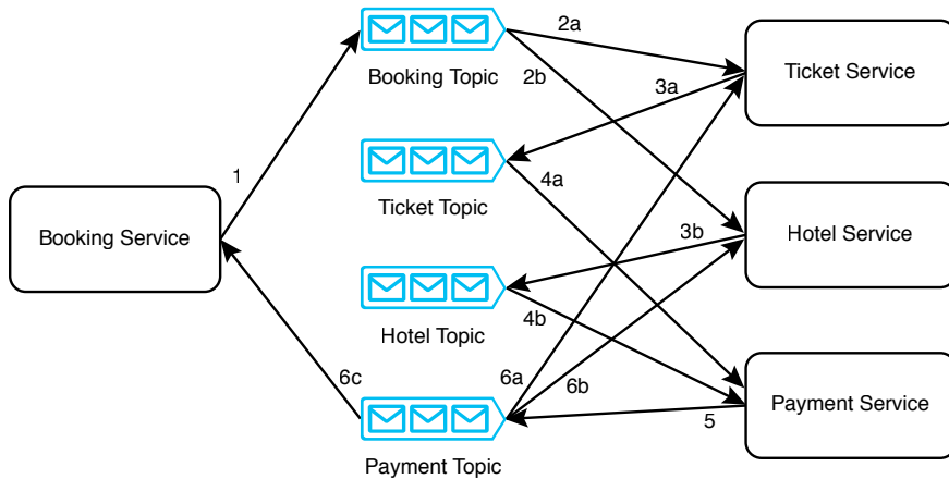
Figure 5.5 A choreography saga to book an airline ticket and a hotel room for a tour package. Two labels with the same number but different letters represent steps that occur in parallel.
