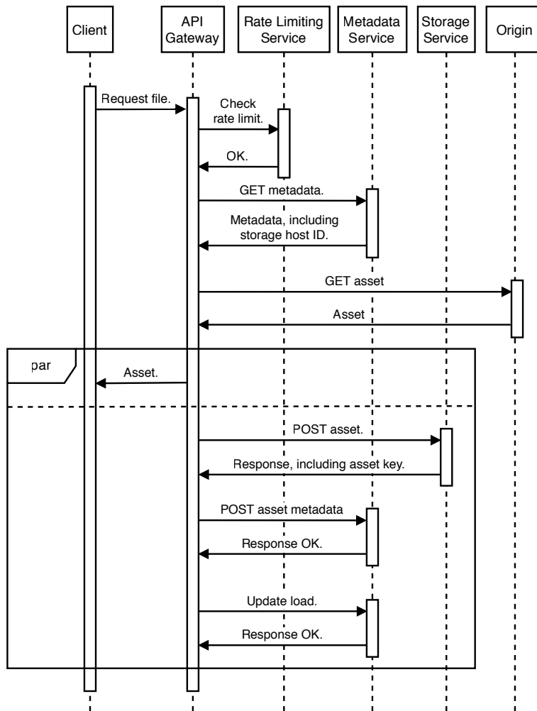
Figure 13.4 Sequence diagram of a CDN download process if the CDN does not contain the requested asset. The CDN will need to download the asset from the origin (a backup location provided by the customer), and return it to the user, as well as store the asset for future requests. POST asset metadata and upload load can be done as a single request, but we can keep them as separate requests for simplicity.
