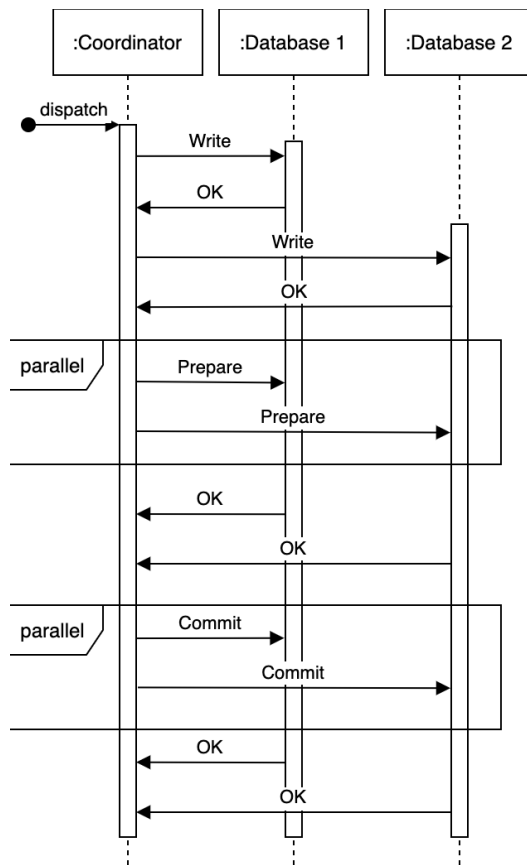
Figure D.1 A successful 2PC execution. This figure illustrates two databases, but the same phases apply to any number of databases. Figure adapted from Designing Data-Intensive Applications by Martin Kleppmann, 2017, O'Reilly Media.
