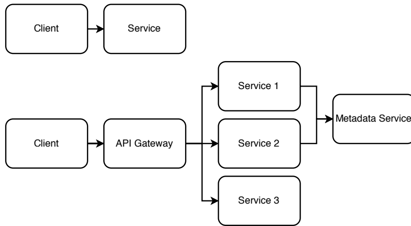
Figure 6.3 Functional partitioning of a service (top) to separate out the API gateway and metadata service (bottom). Before this partitioning, clients query the service directly. With the partitioning, clients query the API gateway, which performs some functions and may route the request to one of the services, which in turn may query the metadata service for certain shared functionalities.
