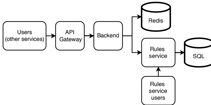
Figure 8.2 Initial high-level architecture of rate limiter. The frontend, backend, and Rules service also log to a shared logging service; this is not shown here. The Redis database is usually implemented as a shared Redis service, rather than our service provisioning its own Redis database. The Rules service users may make API requests to the Rules service via a browser app.
