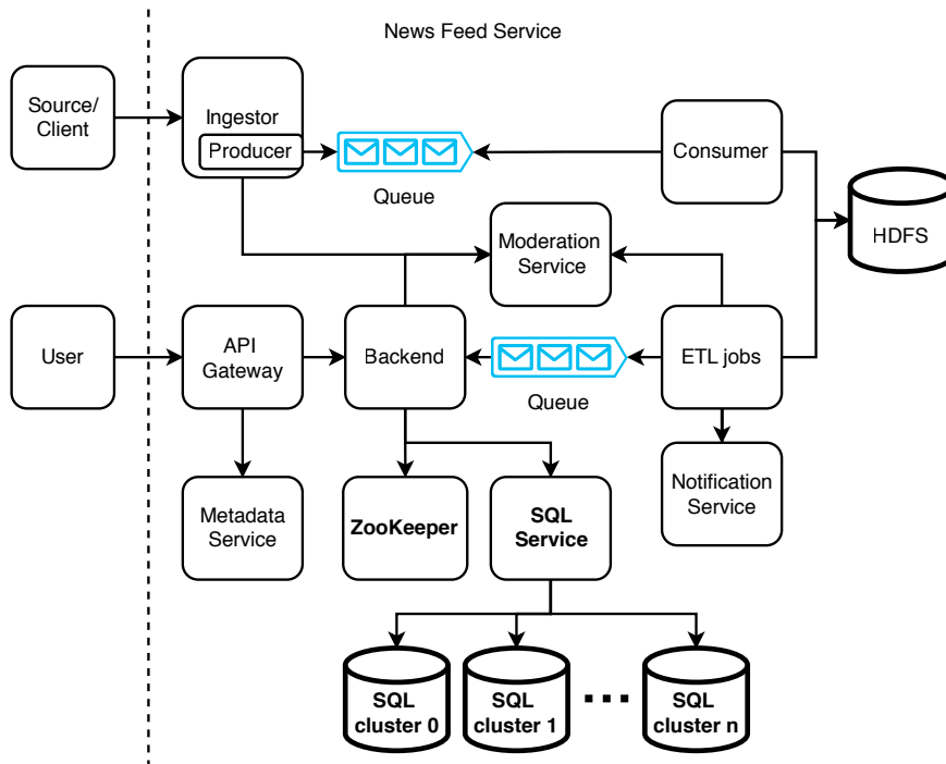
Figure 16.7 High-level architecture of our news feed service with user feeds prepared in advance. Differences from figure 16.4 are bolded . When a user request arrives at our backend, our backend first obtains the appropriate SQL cluster name and then queries the appropriate SQL cluster for the posts. Our backend can direct user requests to a follower node that contains the requested user ID. Alternatively, as illustrated here, we can separate the routing of SQL requests into an SQL service.
