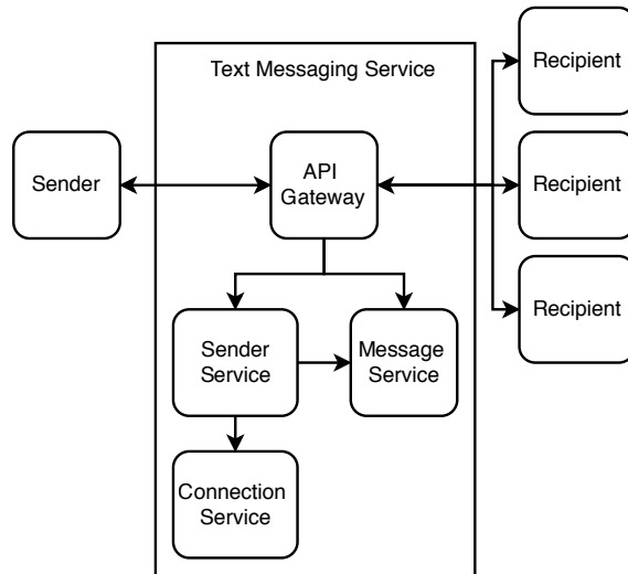
Figure 14.1 High-level architecture with the relationships between our services. A recipient can make requests to send delivery confirmations and read receipts, which are sent to the sender. Any user (sender or receiver) can request the message service for old or undelivered messages.
