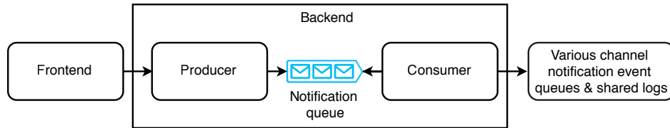
Figure 9.3 Zoom-in of our backend service from figure 9.2. The backend service consists of a producer cluster, a notification Kafka topic, and a consumer cluster. In subsequent illustrations, we will omit the zoom-in diagram of the backend service.
