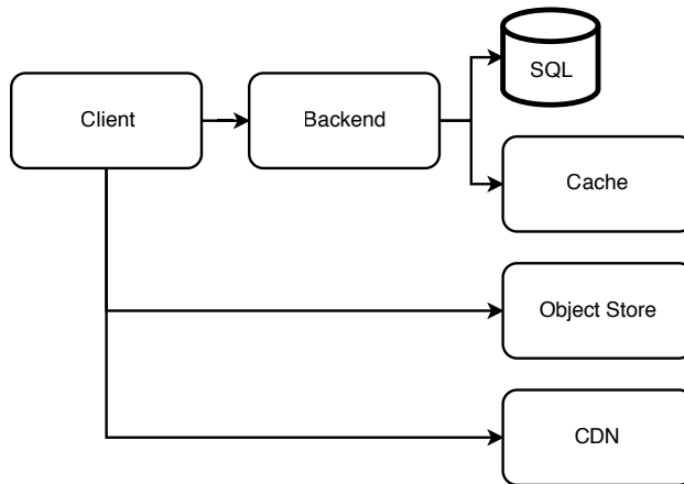
Figure 7.7 Our Craigslist architecture diagram after adding our cache and CDN
