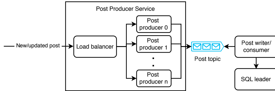
Figure 7.8 Using horizontal scaling and a message broker to handle write traffic spikes
