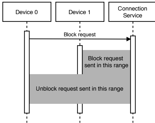
Figure 14.3 If multiple devices can send requests to the connection service, inconsistency may result. If device 0 makes a blocking request followed by an unblocking request, while device 1 makes a blocking request after device 0, it is unclear if the user's intention is to block or unblock.
