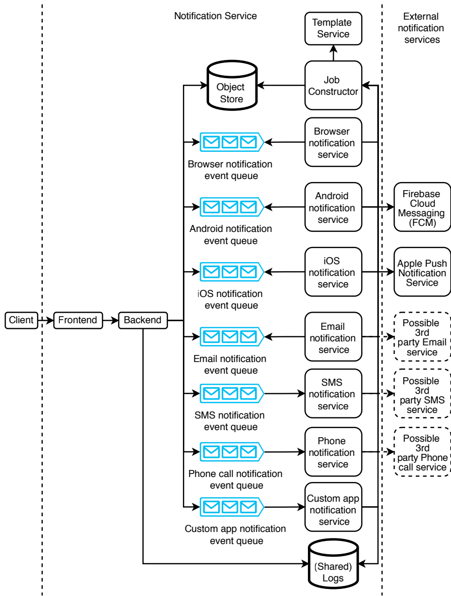
Figure 9.6 High-level architecture including our template service. Notification service users can CRUD templates. The template service should have its own authentication and authorization and RBAC (role-based access control). The job constructor should only have read access. Admins should have admin access so they can create, update, and delete templates or grant roles to other users.
