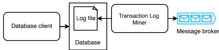
Figure 5.3 Illustration of the transaction log tailing pattern. A service does a write query to a database, which records this query in its log file. The transaction log miner tails the log file and picks up this query, then produces an event to the message broker.
