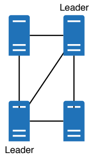
Figure 8.11 Random leader selection may cause multiple leaders to be elected. This will cause unnecessary messaging overhead but does not present other problems.
