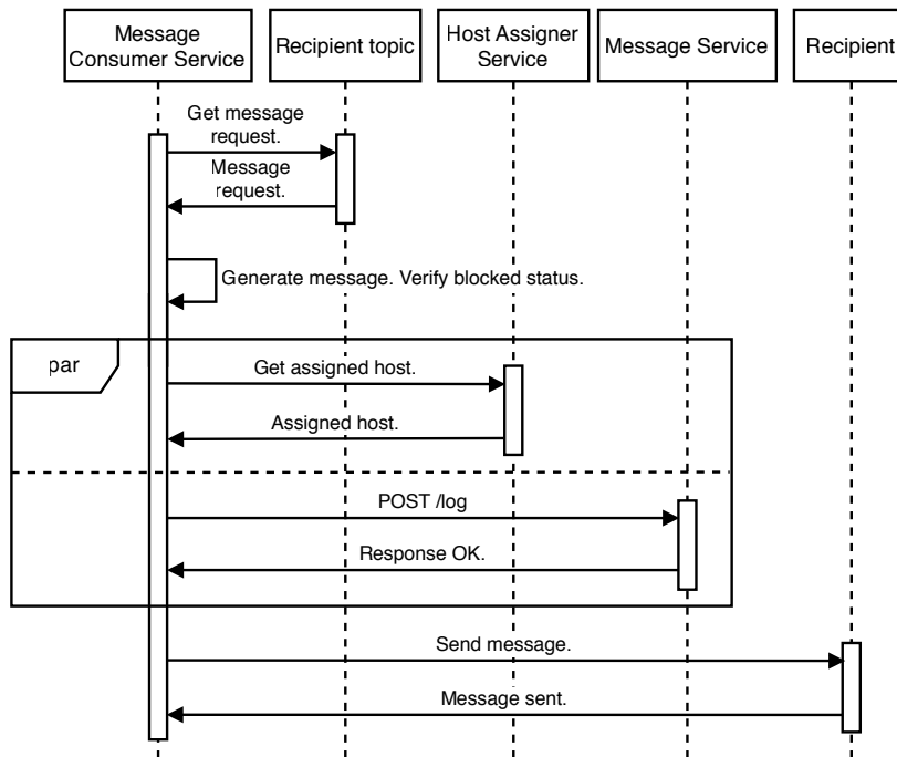
Figure 14.7 Sequence diagram of consuming a message from the recipient Kafka topic and then sending it to our recipient
