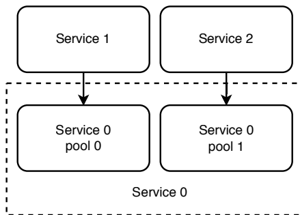
Figure 3.2 Service 0 is divided into two pools, each allocated to a requestor. The unavailability of one pool will not affect the other.
