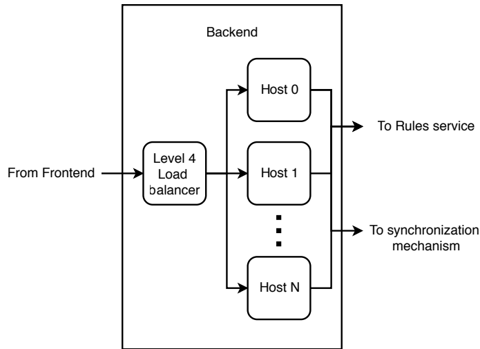
Figure 8.7 High-level architecture of a rate-limiting service where all user request timestamps can fit into a single backend host, requests are randomly load balanced across hosts, and each host can respond to a user request with a rate limiting decision without first making requests to other services or hosts. Hosts synchronize their timestamps with each other in a separate process.
