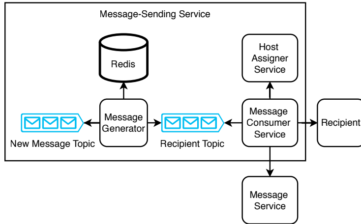
Figure 14.6 High-level architecture of our message-sending service. The message consumer service may go through other services to send the message to the recipient, instead of directly sending it to the recipient as illustrated here.
