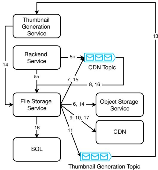
Figure 12.5 Choreography of thumbnail generation, starting from step 5a. The arrows indicate the step numbers described in the main text. For clarity, we didn't illustrate the user. Some of the events that the file storage service produces and consumes to the Kafka topics are to signal it to transfer image files between the object storage service and the CDN. There are also events to trigger thumbnail generation, and to write CDN metadata to the SQL service.
