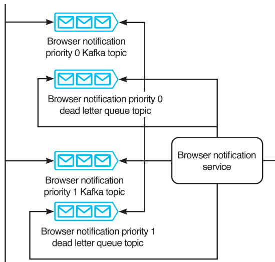
Figure 9.13 Figure 9.12 with two priority levels
