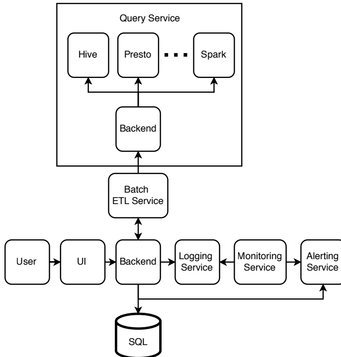
Figure 10.4 Revised high-level architecture with a shared query service through which other services make database requests.
