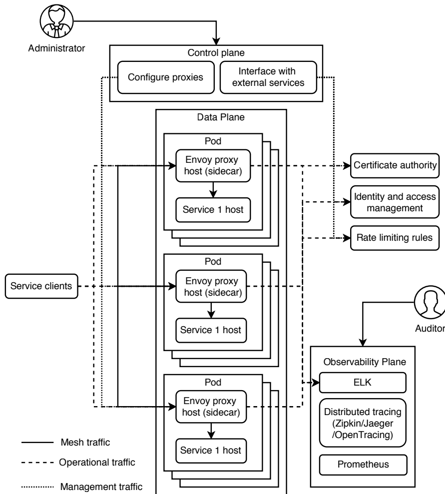
Figure 1.8 Illustration of a service mesh. Prometheus makes requests to each proxy host to pull/scrape metrics, but this is not illustrated in the diagram because the many arrows will make it too cluttered and confusing. Figure adapted from https://livebook.manning.com/book/cloud-native/chapter-10/146 .
