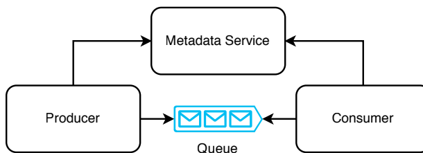
Figure 6.2 We can use a metadata service to reduce the size of individual messages in a queue, by placing large objects in the metadata service, and enqueueing only IDs in individual messages.
