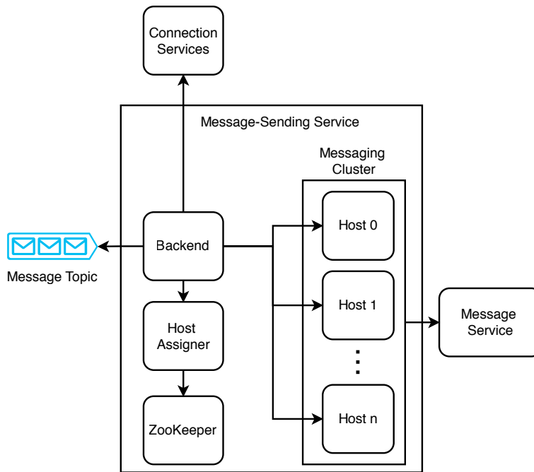
Figure 14.8 High-level architecture of the message-sending service that assigns clients to dedicated hosts. Message backup is not illustrated.
