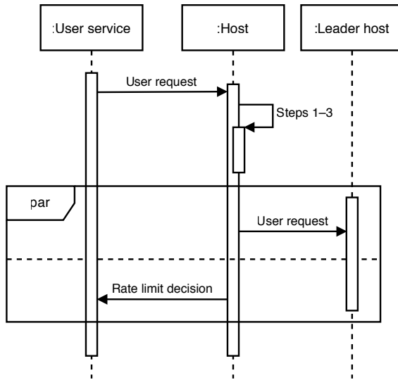
Figure 8.15 Sequence diagram of our fixed window counter approach. This diagram illustrates the approach of using the host’s memory to store the request timestamps, instead of Redis. The rate-limiting decision is made immediately on the host, using only data stored in the host’s memory. The subsequent steps on the leader host for synchronization are not illustrated.
