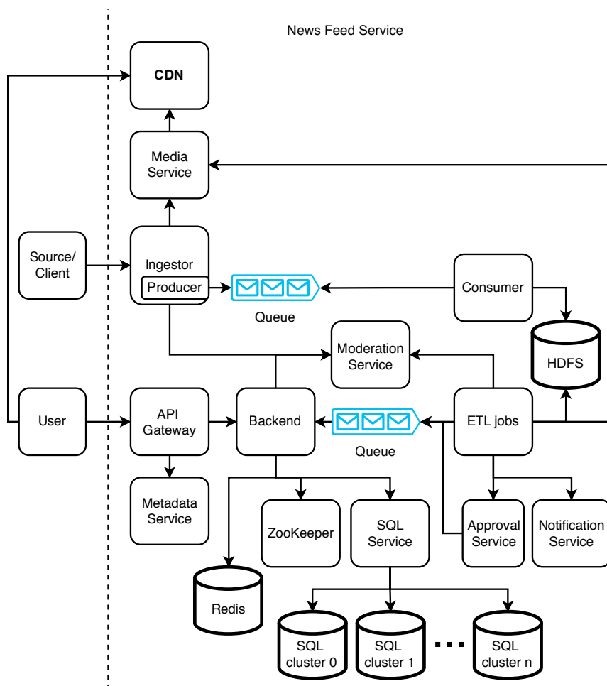
Figure 16.12 Using a CDN (in bold; this service is added to figure 16.10) to host media. Users will download images directly from our CDN, gaining the benefits of a CDN such as lower latency and higher availability.
