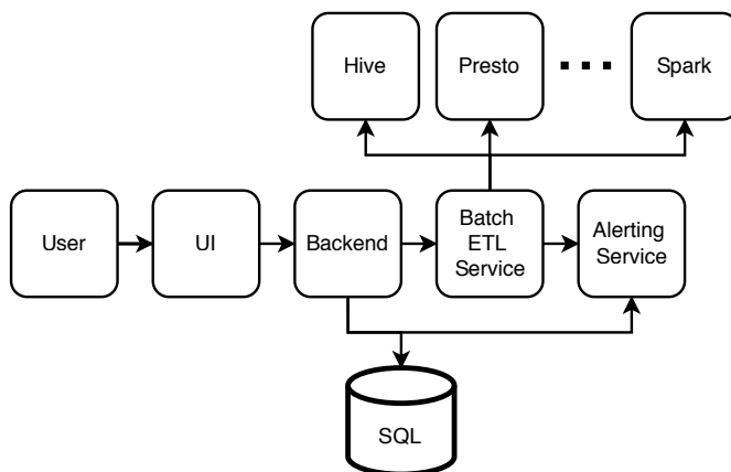
Figure 10.1 Initial high-level architecture of a hypothetical service for users to define periodic validation checks on their data.
