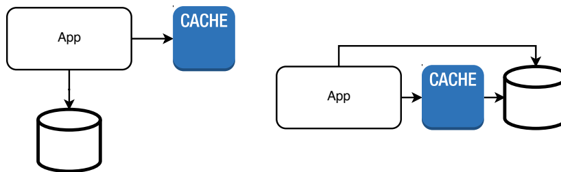
Figure 4.12 Two possible architectures of write-around. (Left) Write-around with cache-aside. (Right) Write-around with read-through.
