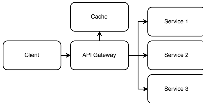
Figure 4.9 Caching at an API gateway. Diagram adapted from Rob Vettor, David Coulter, Genevieve Warren. May 17, 2020. “Caching in a cloud-native application.” Microsoft Docs. https://docs.microsoft.com/en-us/dotnet/architecture/cloud-native/azure-caching .
