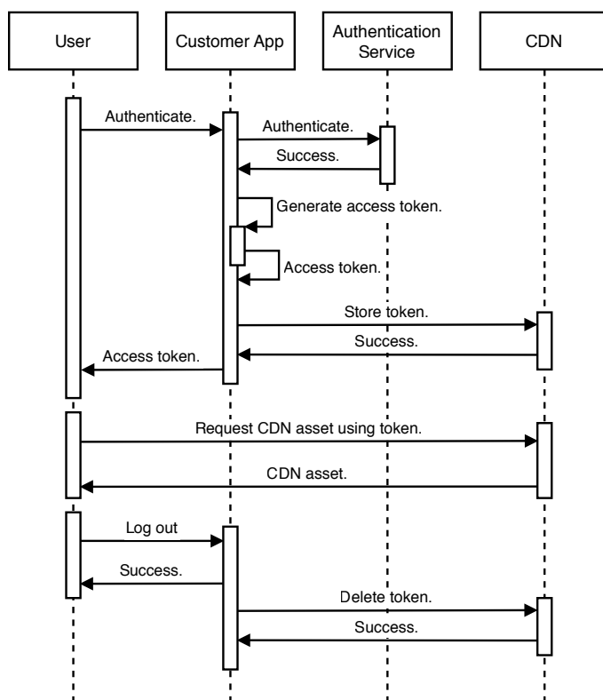
Figure 13.1 Sequence diagram of token generation process, followed by using the token to request CDN assets, and destroying the token upon user logout. The process of destroying the token can be asynchronous as illustrated here, or it can be synchronous because logouts are not frequent events.
