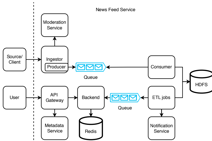
Figure 16.2 High-level architecture of our news feed service. A client submits a post to our news feed service. Our ingestor receives the post and performs some simple validations. If the validations pass, our ingestor produces it to a Kafka queue. Our consumer cluster consumes the post and writes it to HDFS. Our batch ETL jobs process the posts and produce them to another Kafka queue. They may also trigger notifications via a notification service. User requests for posts go through our API gateway, which may retrieve users' tags from our metadata service and then retrieve posts from our Redis table via our backend service. When backend hosts are idle, they consume from the queue and update the Redis table.
