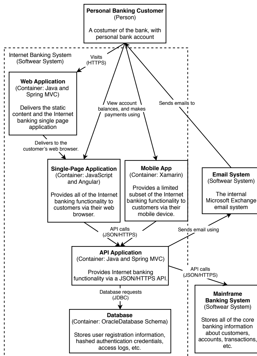
Figure C.2 A container diagram. Adapted from https://c4model.com/ , licensed under https://creativecommons.org/licenses/by/4.0/ .
