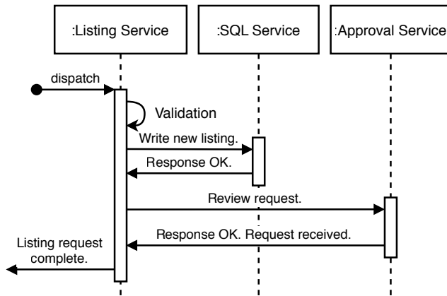
Figure 15.3 Sequence diagram of a simplified request to create or update a listing
