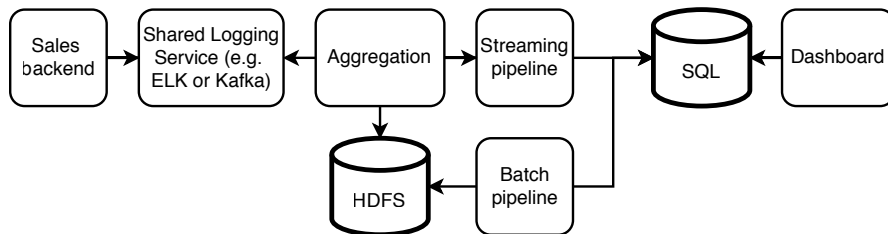
Figure 17.2 Our Lambda architecture, consisting of an initial aggregation service and streaming and batch pipelines. Arrows indicate the direction of requests. The sales backend logs events (including sales events) to a shared logging service, which is the data source for our dashboard. Our aggregation service consumes sales events from our shared logging service, aggregates them, and flushes these aggregated events to our streaming pipeline and to HDFS. Our batch pipeline computes the counts from our HDFS data and writes it to the SQL batch_table. Our streaming pipeline computes the counts faster and less accurately than our batch pipeline and writes it to the SQL speed_table. Our dashboard uses a combination of data from batch_table and speed_table to generate the Top K lists.
