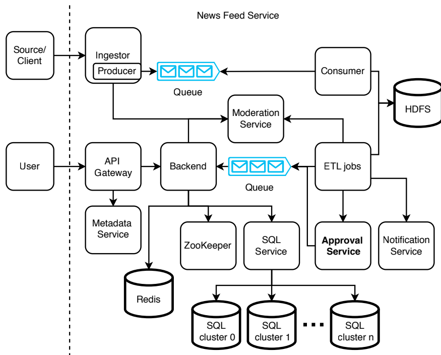
Figure 16.9 ETL jobs can flag certain posts for manual approval. These posts can be sent to our approval service (in bold; this service is added to figure 16.8) for manual review, instead of being produced by a Kafka queue. (If we have a high rate of posts flagged for review, our approval service itself may need to contain a Kafka queue.) If a reviewer approves a post, it will be sent back to our Kafka queue via an ETL job to be consumed by our backend (or it can send the post directly to our backend). If a reviewer rejects a post, our approval service can notify the source/client via a messaging service, not illustrated in this figure.
