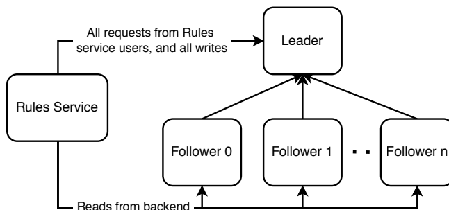
Figure 8.3 The leader host should process all requests from Rules service users, and all write operations. Reads from the backend can be distributed across the follower hosts.
