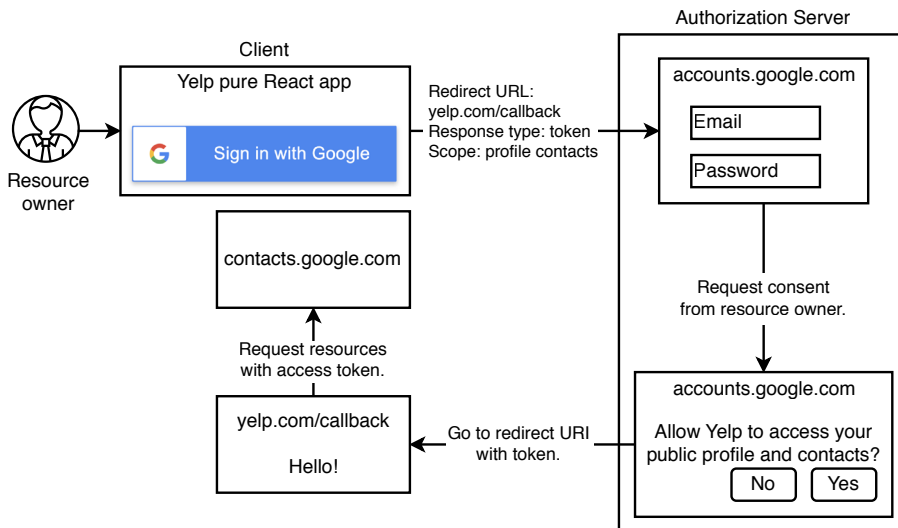
Figure B.3 Illustration of an OAuth2 implicit flow. All communications are front channel. Note that the request to the authorization server has response type “token” instead of “code.”
