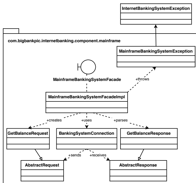
Figure C.4 A code (UML class) diagram. Image adapted from https://c4model.com/ , licensed under https://creativecommons.org/licenses/by/4.0/ .
