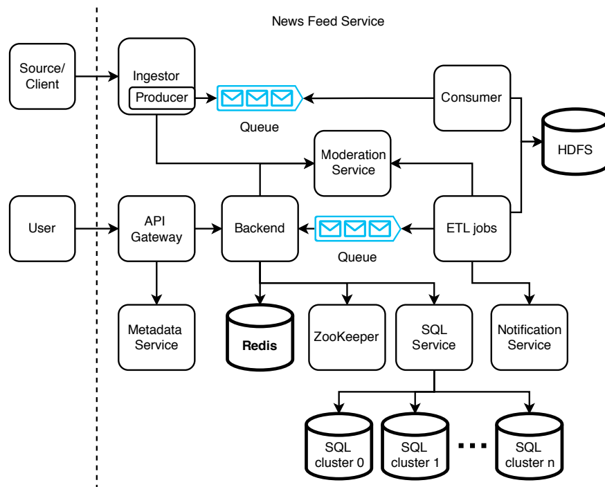
Figure 16.8 High-level architecture with both a prepared feed and Redis service. The difference from figure 16.7 is the added Redis service, which is bolded .
