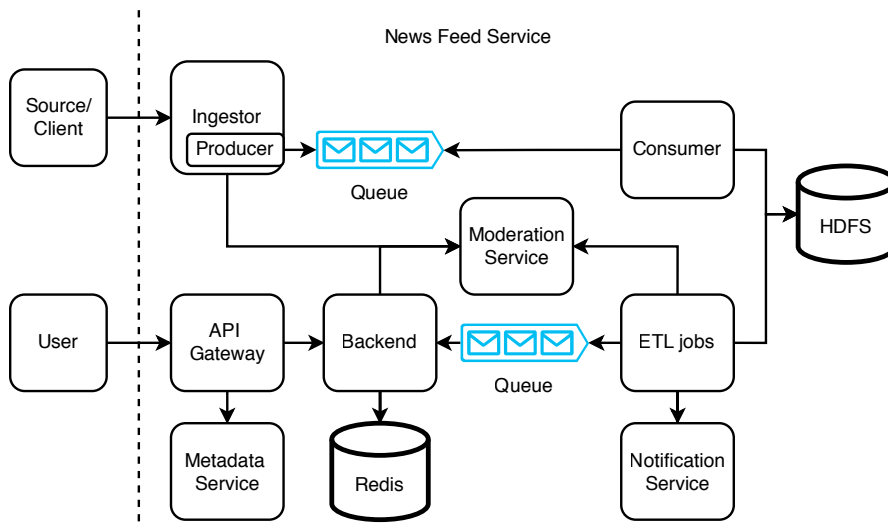
Figure 16.4 High-level architecture of our news feed system with all content moderation centralized in a moderation service. Developers can define all content moderation logic in this service.
