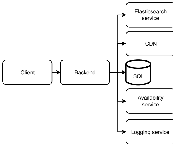
Figure 15.8 High-level architecture of the booking service
