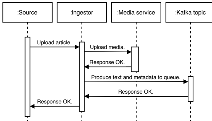
Figure 16.11 Sequence diagram of a source uploading an article. Media is almost always larger than text, so our ingestor first uploads media to our Media Service. After our ingestor successfully uploads the media, it produces the text and metadata to our Kafka topic, to be consumed and written to HDFS as discussed in this chapter.
