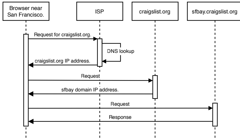
Figure 7.6 Sequence diagram for using GeoDNS to direct user requests to the appropriate IP address
