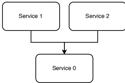
Figure 3.1 All requests to service 0 are load-balanced across its hosts. The unavailability of service 0's hosts will prevent it from serving any requestor.
