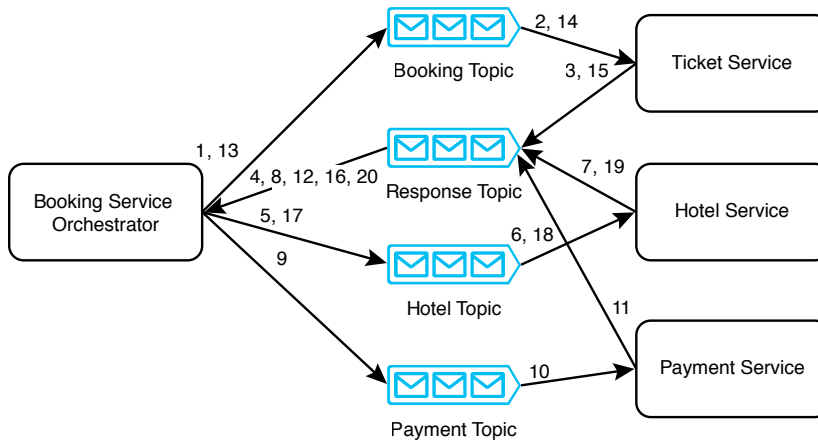
Figure 5.6 An orchestration saga to book an airline ticket and a hotel room for a tour package
